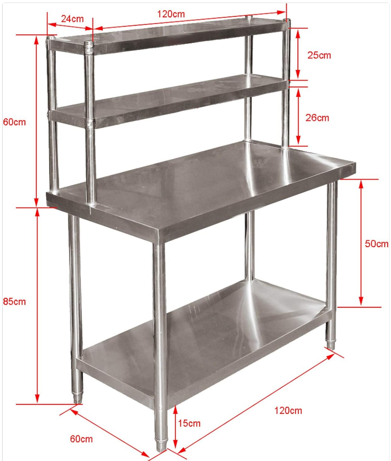
Figure 3.1: Dimensional overview of the WilTec Stainless Steel Work Table, including the main worktop and the 2-tier upper shelf.
