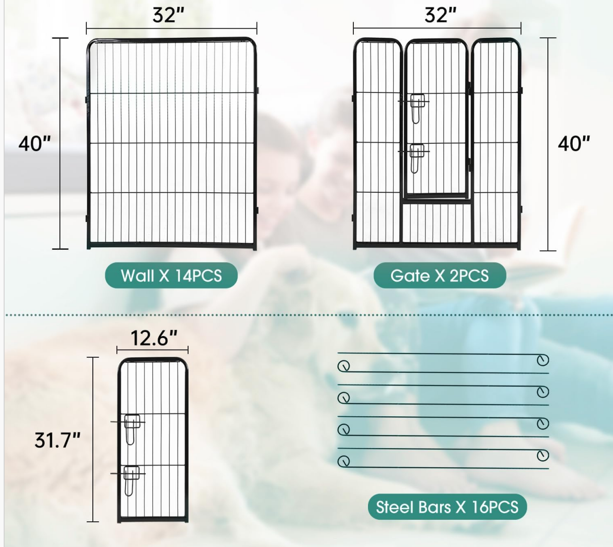
Image 3.1: Visual representation of the playpen components, detailing the dimensions of the wall panels, gate panels, and connecting steel bars.
