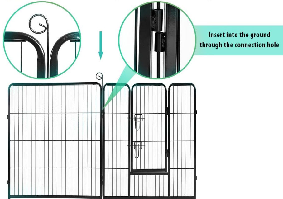
Image 4.1: Step-by-step guide demonstrating the simple process of connecting two playpen panels using a steel bar.
