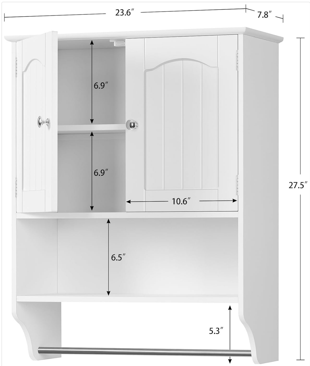
Figure 3.1: Cabinet dimensions for planning installation space.
