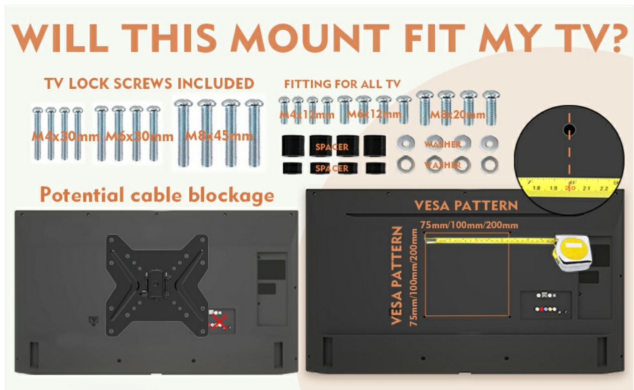
Image 3: Guide for checking TV VESA pattern compatibility and included mounting hardware.
