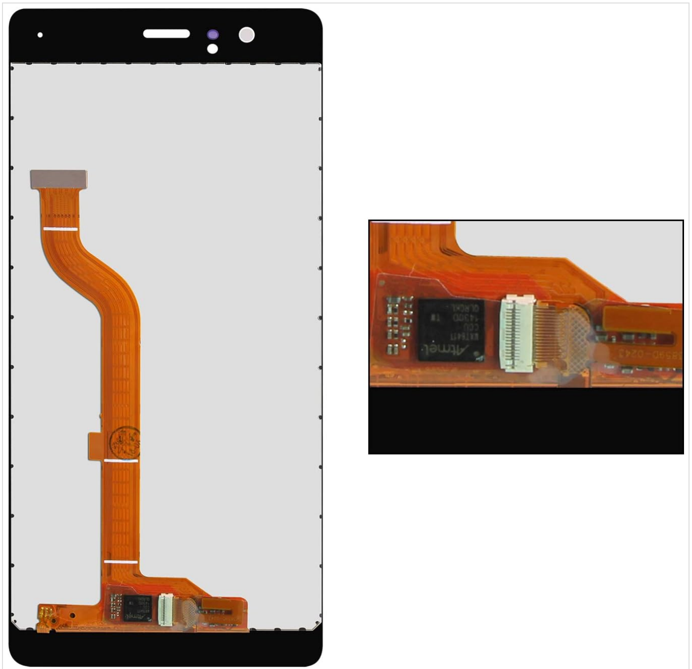
Image 2.2: Detailed view of the flex cable and its connector. Handle this component with care to avoid damage to the delicate circuitry.
