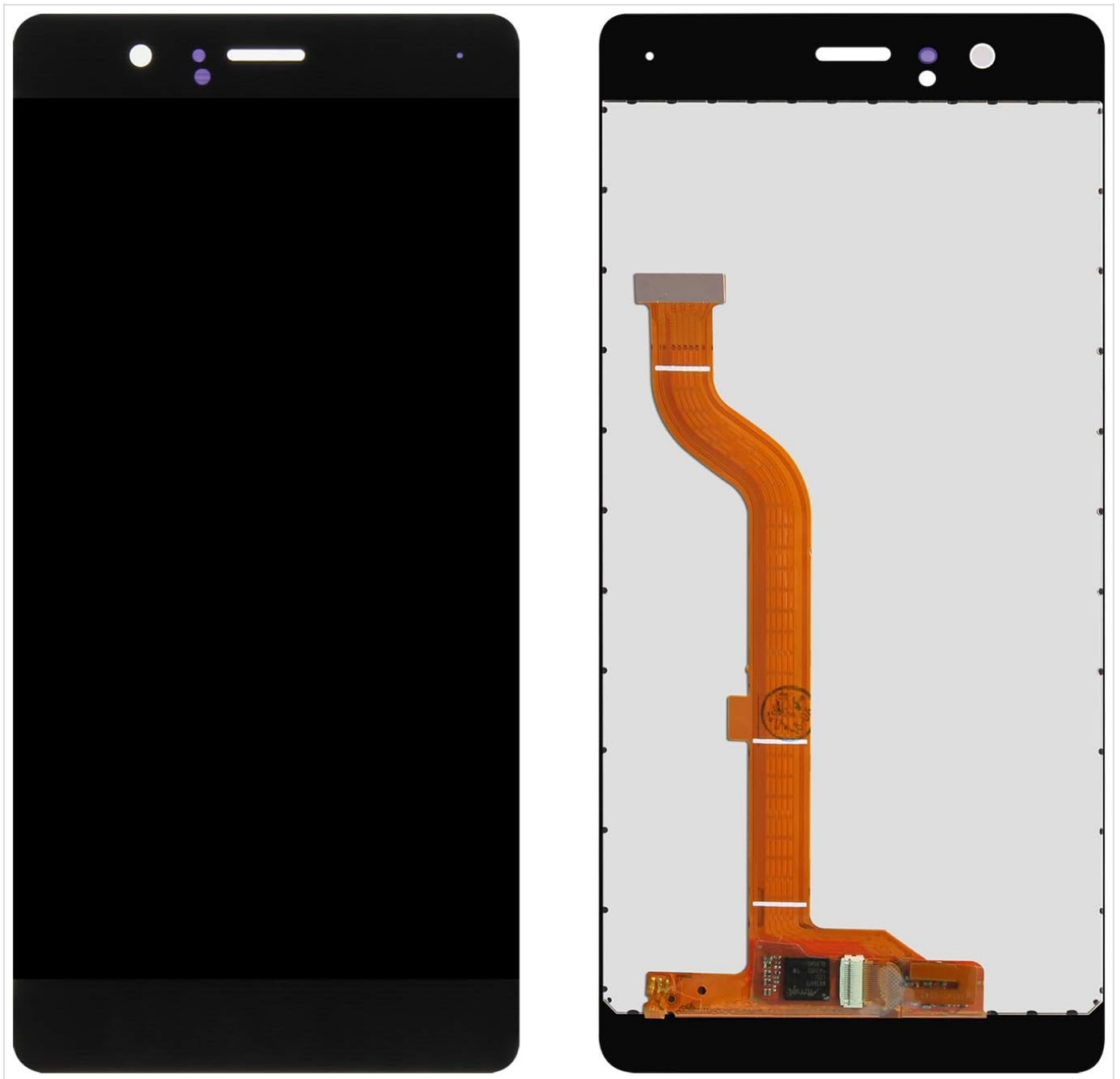
Image 2.1: Front and back view of the replacement LCD screen, highlighting the flex cable connection. Ensure this cable is properly seated and secured during installation.
