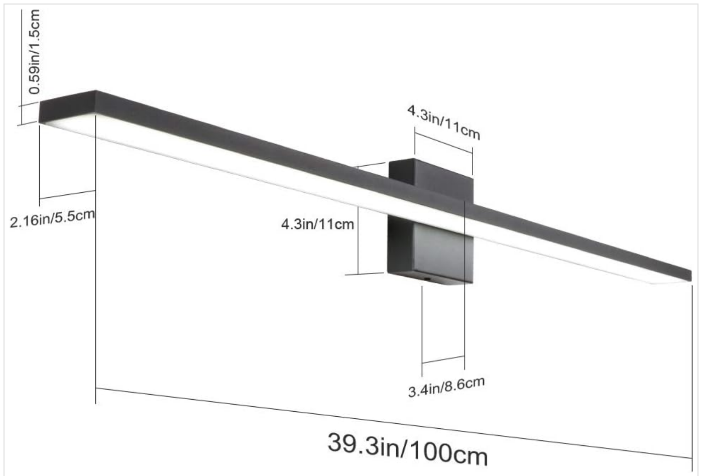
Image 4.2: Detailed dimensions of the light fixture.
