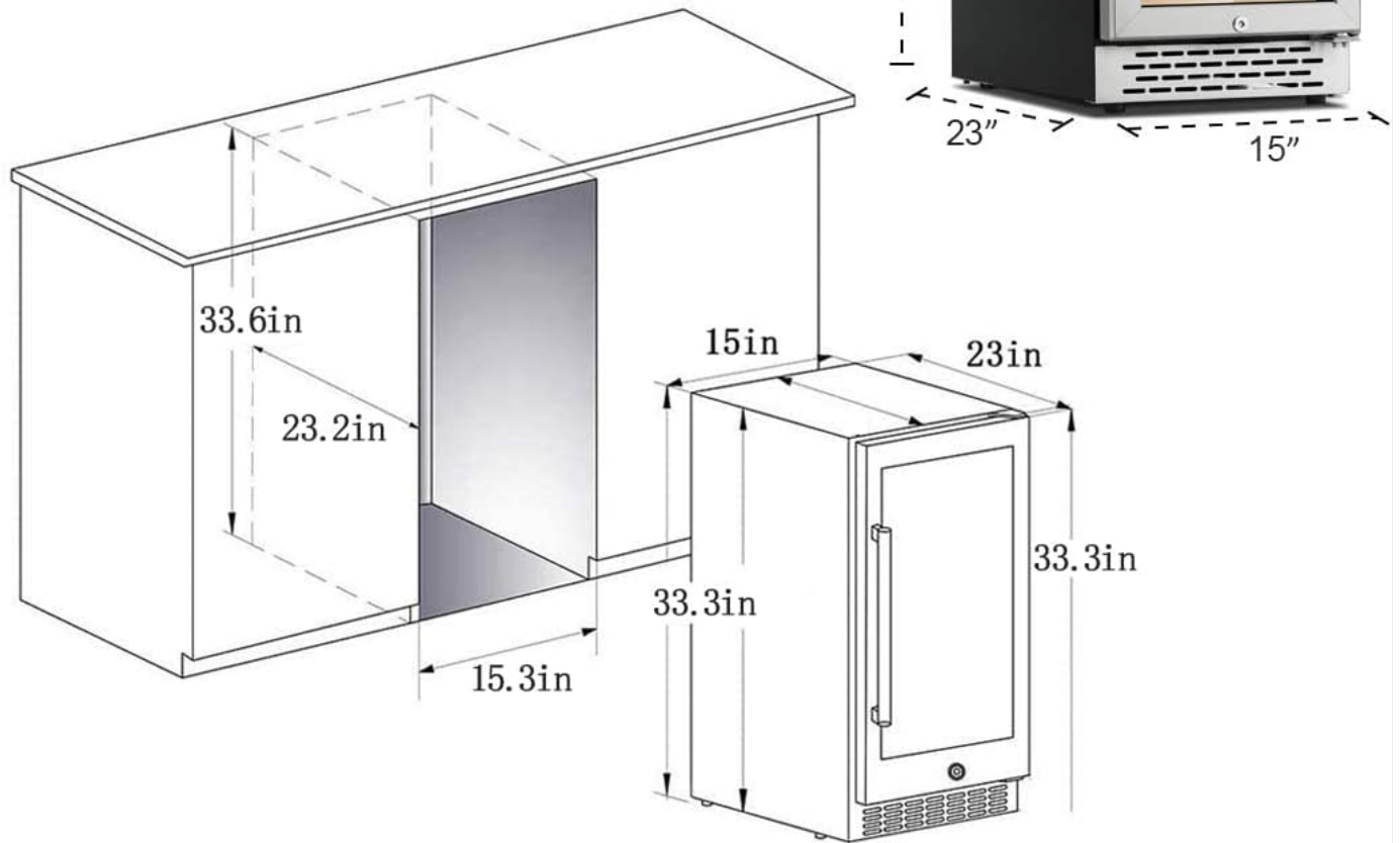
Image: Diagram illustrating the dimensions of the 15-inch wine cooler and examples of both freestanding and built-in installation within cabinetry.
