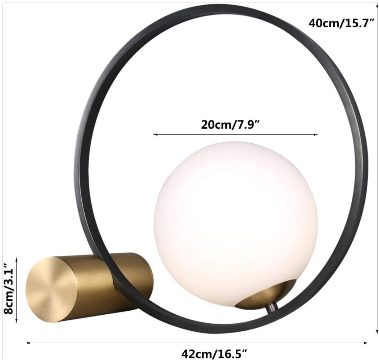
Figure 4: Dimensional overview of the KCO Lighting Table Lamp. This image provides precise measurements for height, width, and globe diameter.
