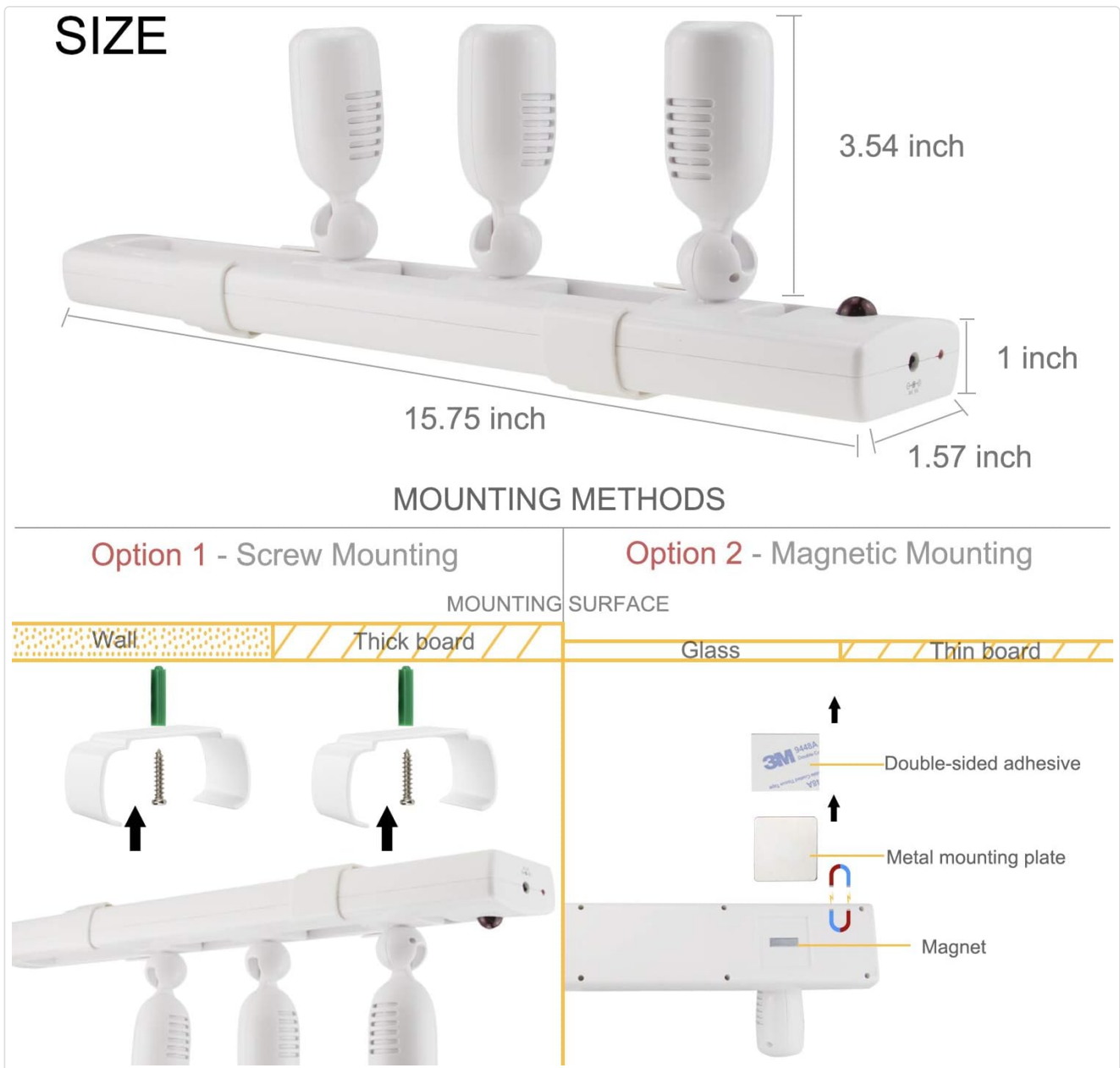
Figure 4.1: Two primary installation methods for the track lighting system. Option 1 demonstrates screw mounting for solid surfaces like walls or thick boards. Option 2 illustrates magnetic mounting, suitable for glass or thin boards, utilizing double-sided adhesive tape and a metal mounting plate.
