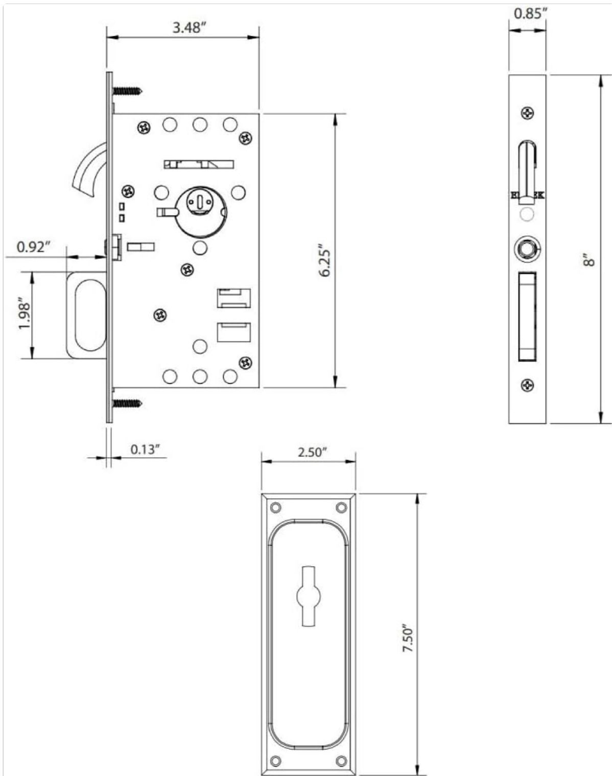
Figure 2: Technical drawing showing dimensions of the Emtex 2105 Mortise Lock body, faceplate, and trim plate. Key dimensions include mortise body height 6.25", width 3.48", faceplate height 8", width 0.85", and trim plate height 7.50", width 2.50".
