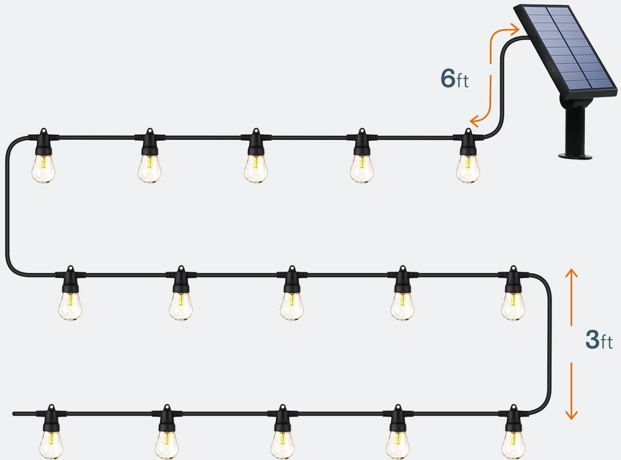
Figure 2: Detailed dimensions of the 48-foot string with 15 LED bulbs, showing 3 feet between each bulb.
