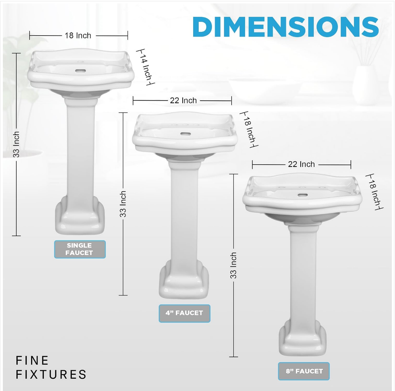
Image: Illustrates the dimensions of various Roosevelt Pedestal configurations, including the 33-inch height relevant to the column.
