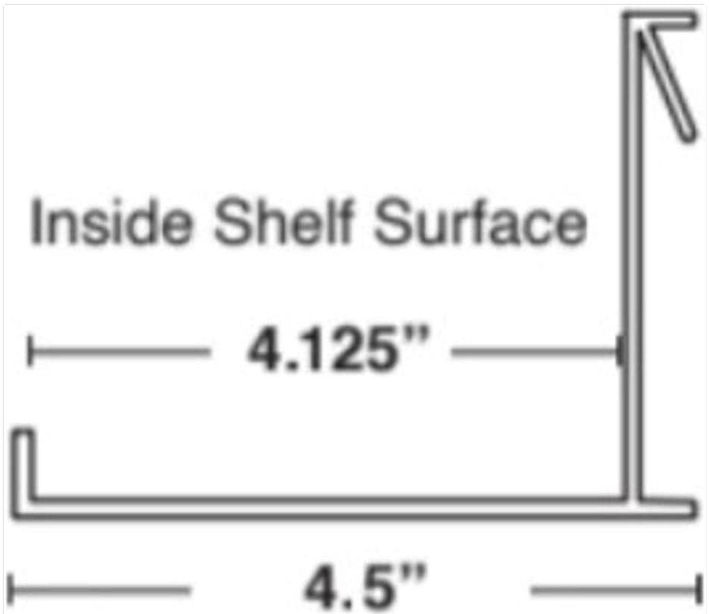
Image: Technical diagram illustrating the shelf's dimensions, including inside shelf surface and total depth.
