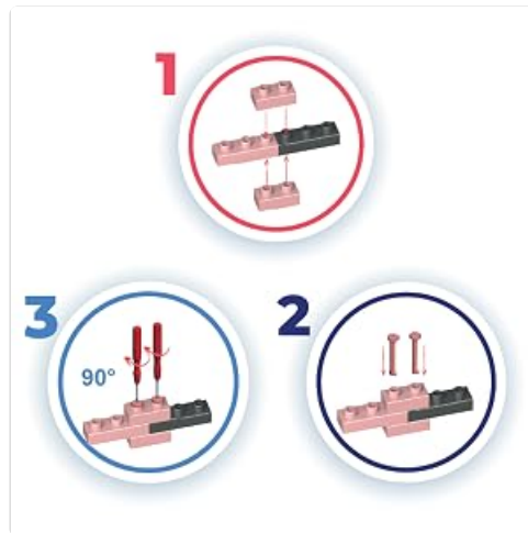
Image: A circular diagram showing three steps for connecting JEKCA bricks. Step 1 illustrates aligning two bricks. Step 2 shows inserting two pins into the aligned bricks. Step 3 depicts using the pin driver to turn the pins 90 degrees for a secure lock.
