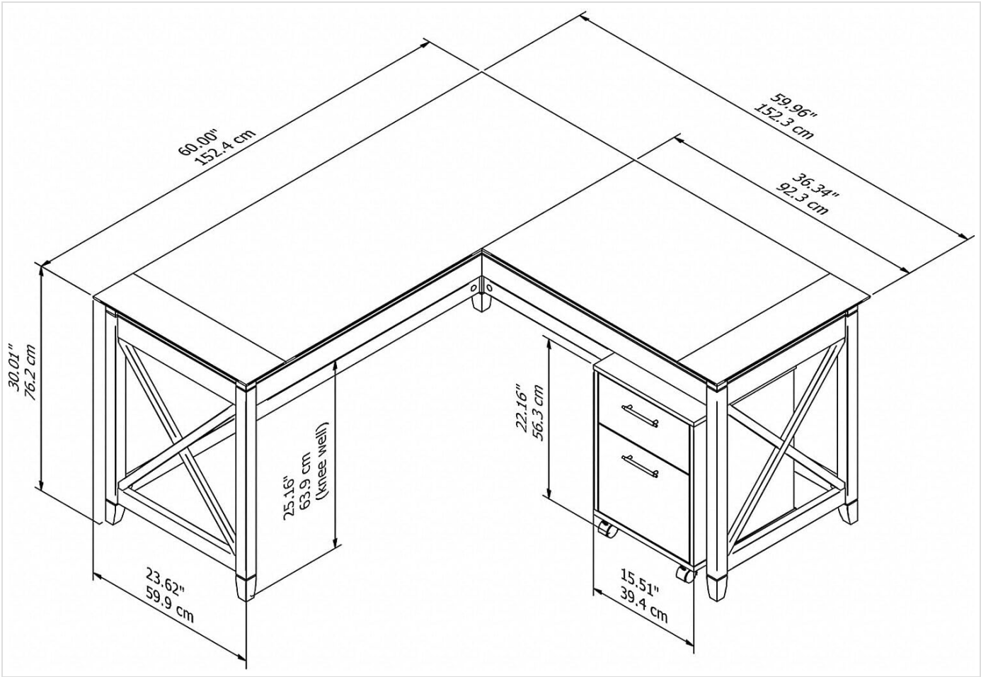
Figure 4.1: Detailed dimensions of the L Shaped Desk and Mobile File Cabinet.
