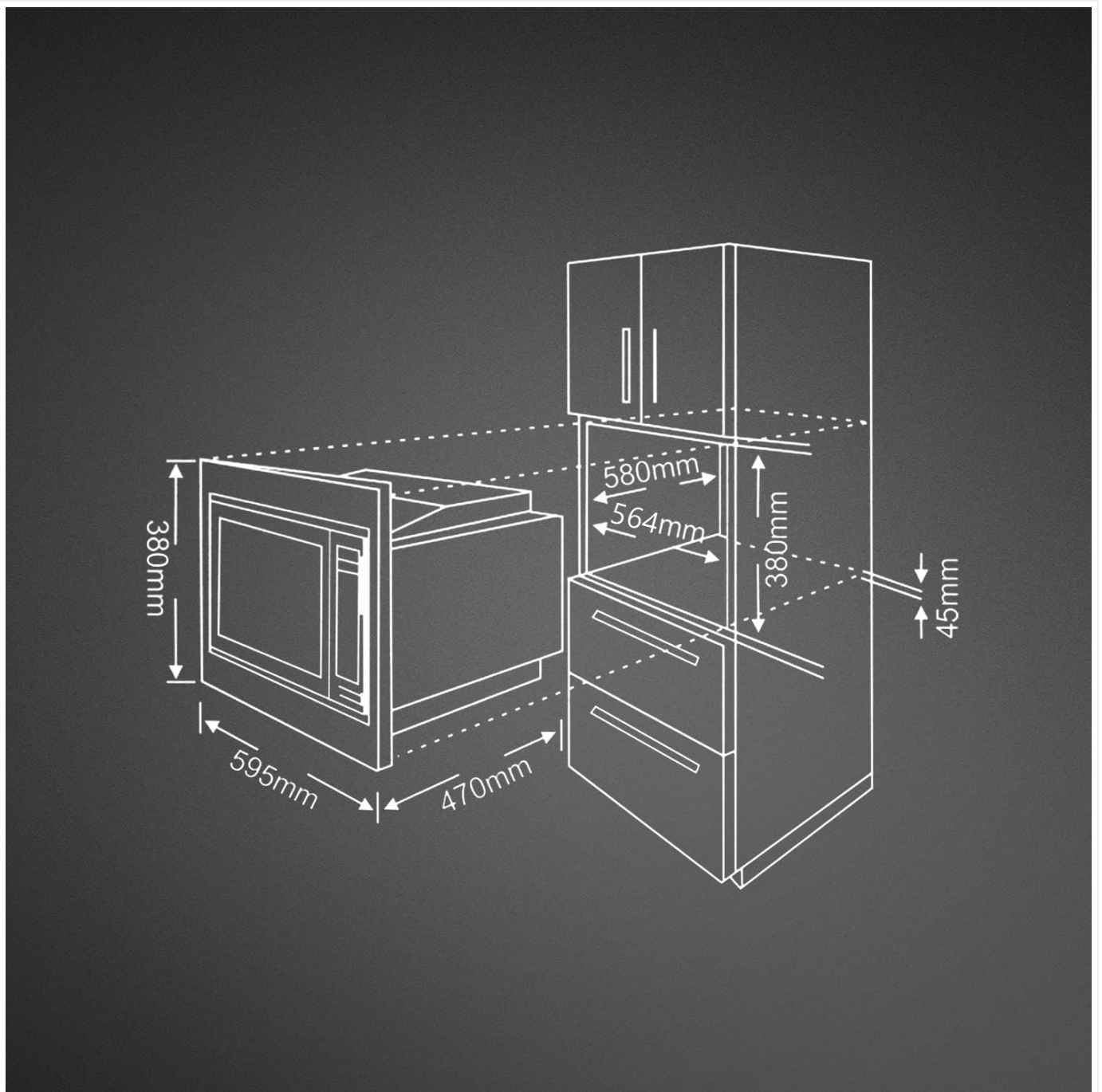
Figure 4: Installation diagram showing required cabinet cut-out dimensions (e.g., 564mm width, 380mm height, 580mm depth).
