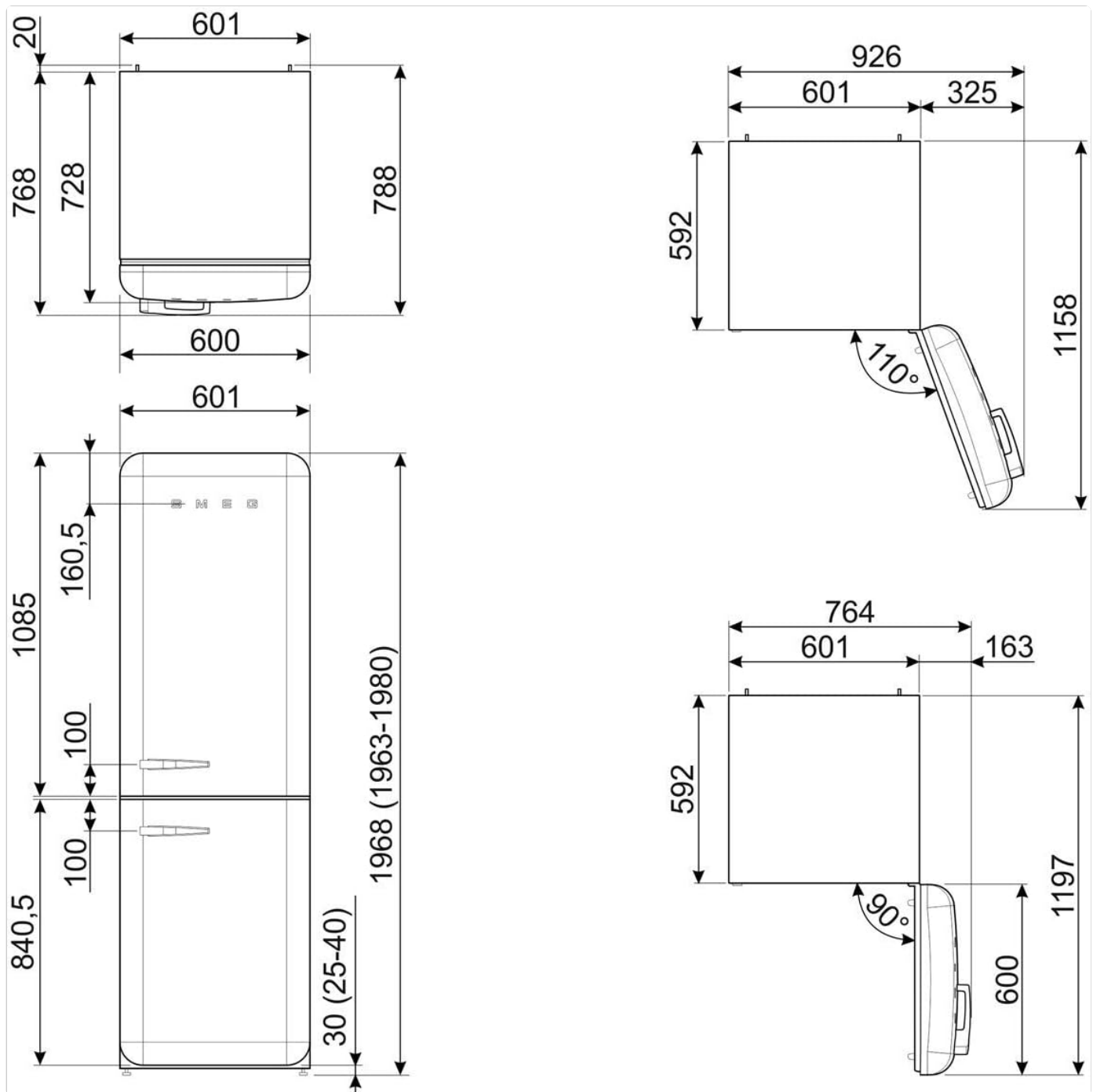
Figure 2: Technical drawing illustrating the dimensions of the SMEG FAB32URPG3 refrigerator. This diagram provides measurements for height, width, depth, and door opening clearances, crucial for proper installation planning.
