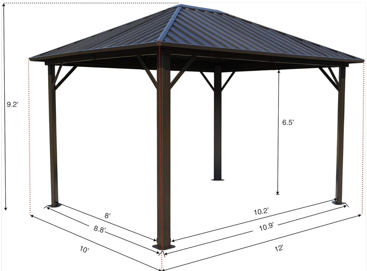
Detailed dimensions of the gazebo, including height and footprint measurements.
