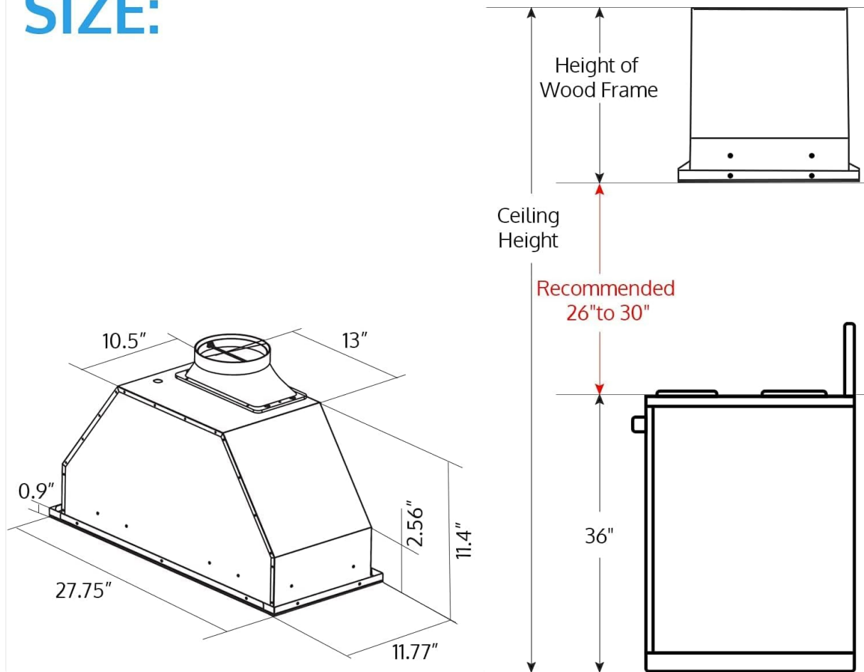
Figure 6: Dimensional drawing of the range hood, including recommended installation height above the cooking surface (26" to 30").
