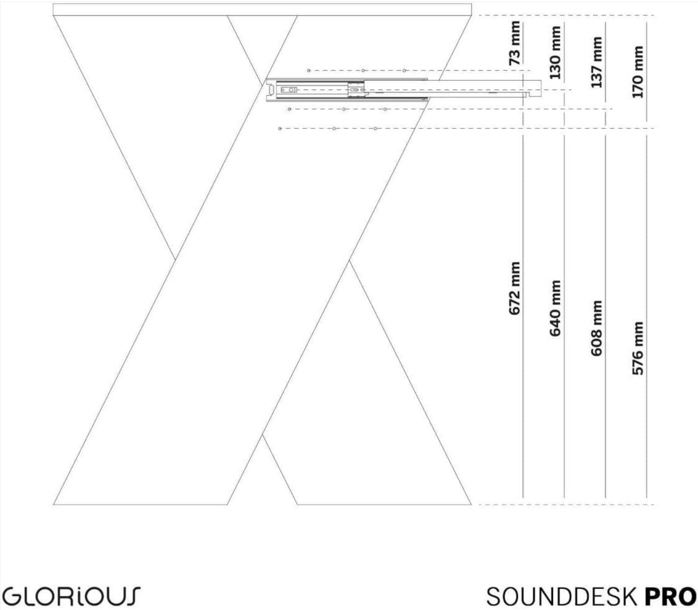
Figure 4.1: Keyboard tray height adjustment options (measurements in mm).
