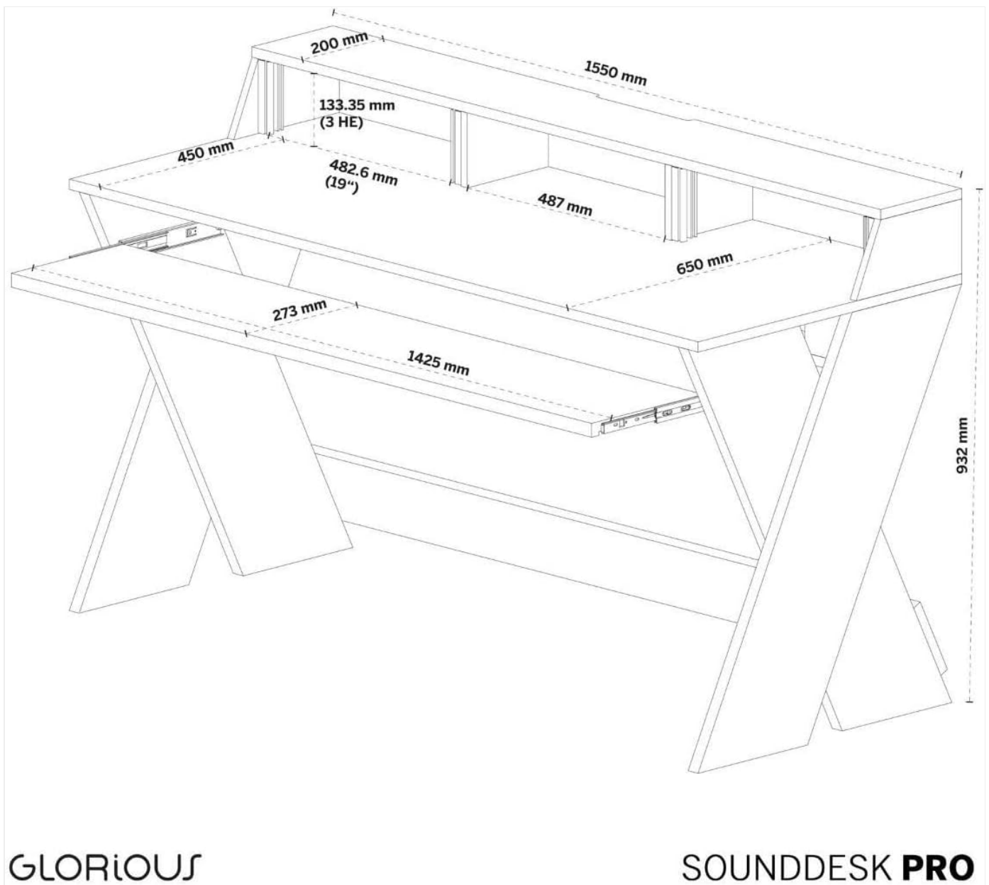
Figure 4.2: Overall dimensions of the Glorious Sound Desk Pro (measurements in mm).
