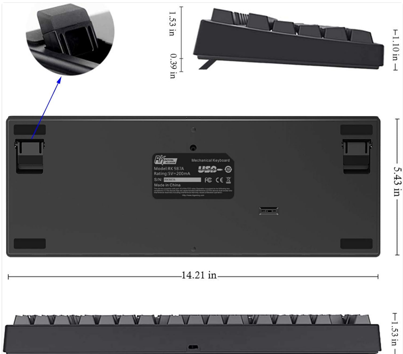
Figure 4.1: Detailed dimensions and model information located on the keyboard's underside.
