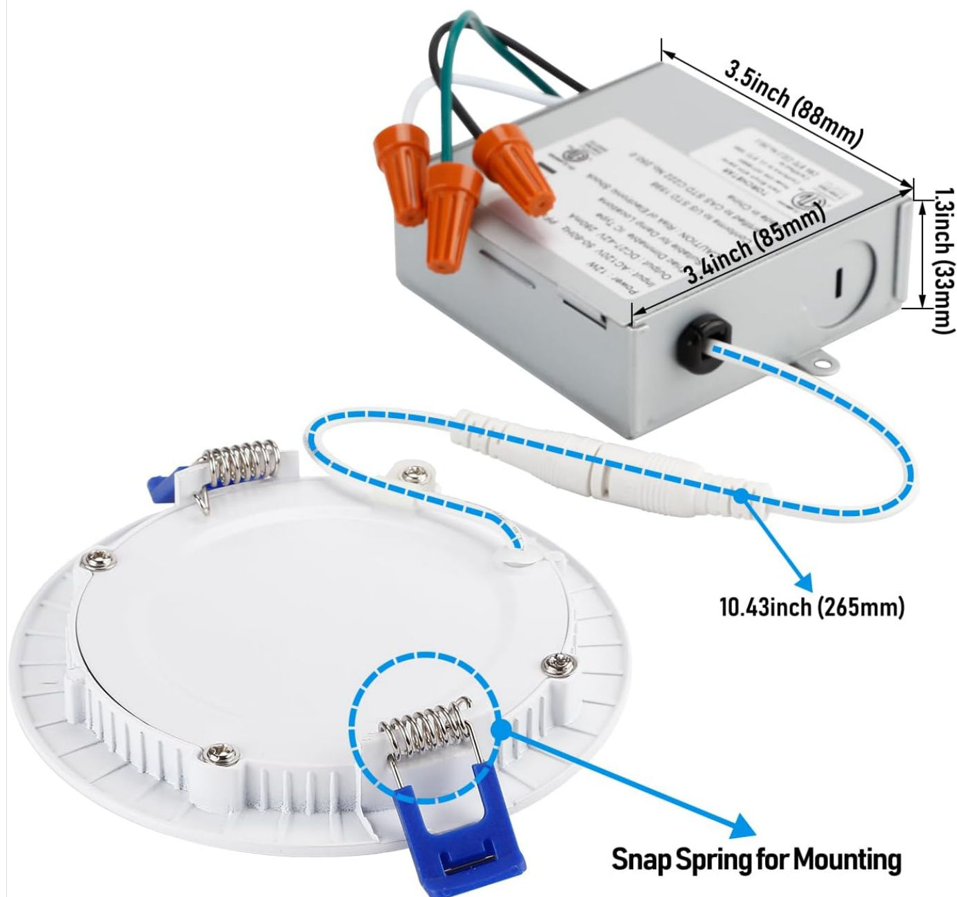
Image 6.1: Product dimensions and cut-out hole size for installation.
