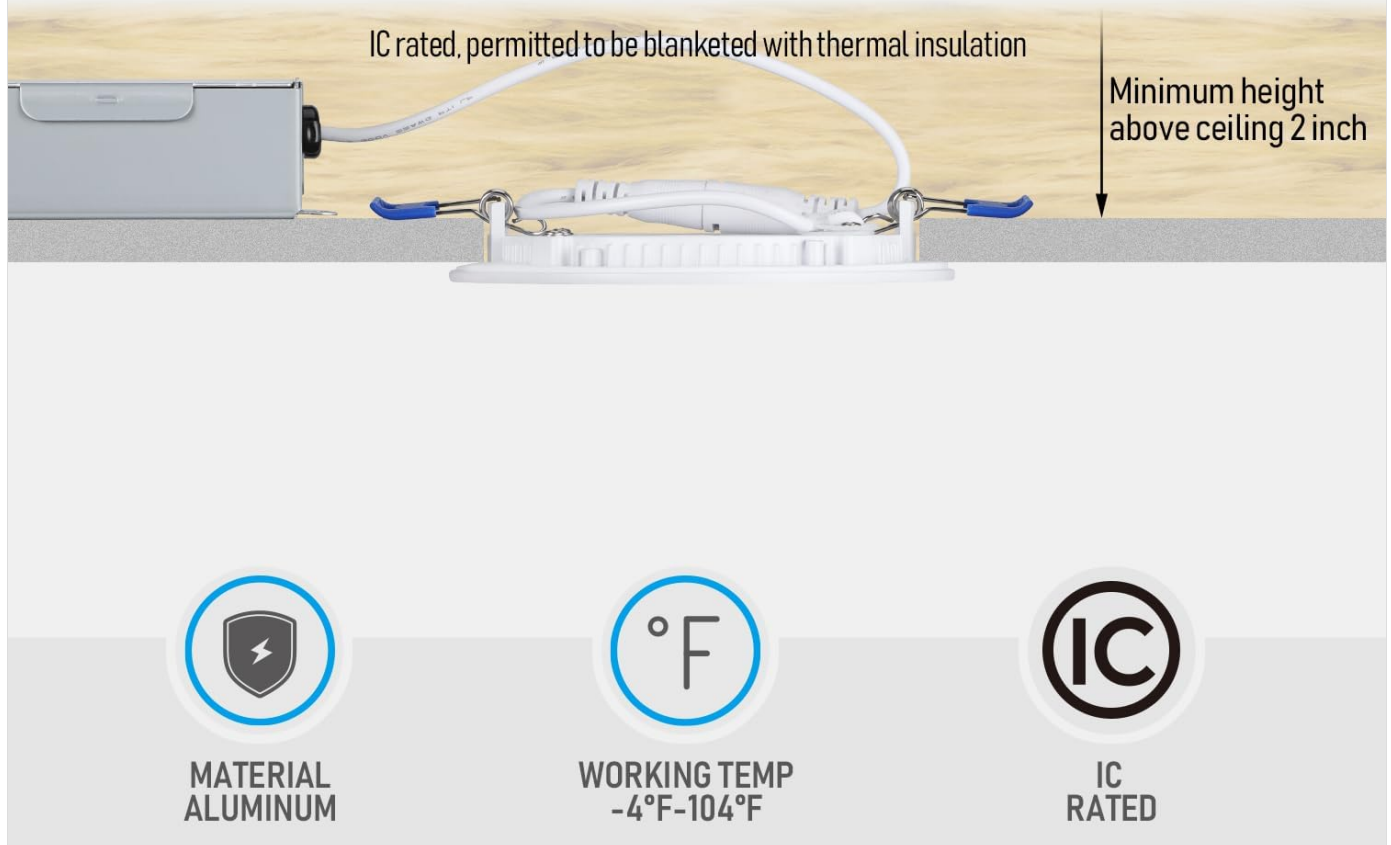
Image 6.3: The ultra-thin design allows installation in tight ceiling spaces and is IC-rated for contact with insulation.
