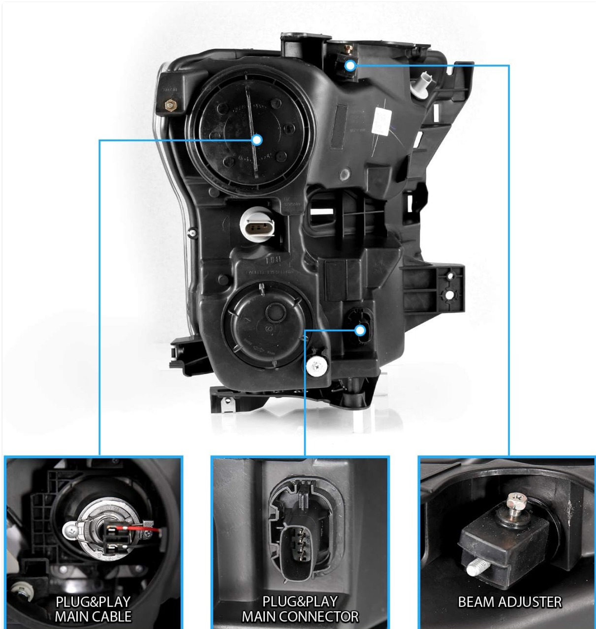
Rear view of the headlight assembly highlighting the plug-and-play main cable, main connector, and the beam adjuster for precise light alignment.
