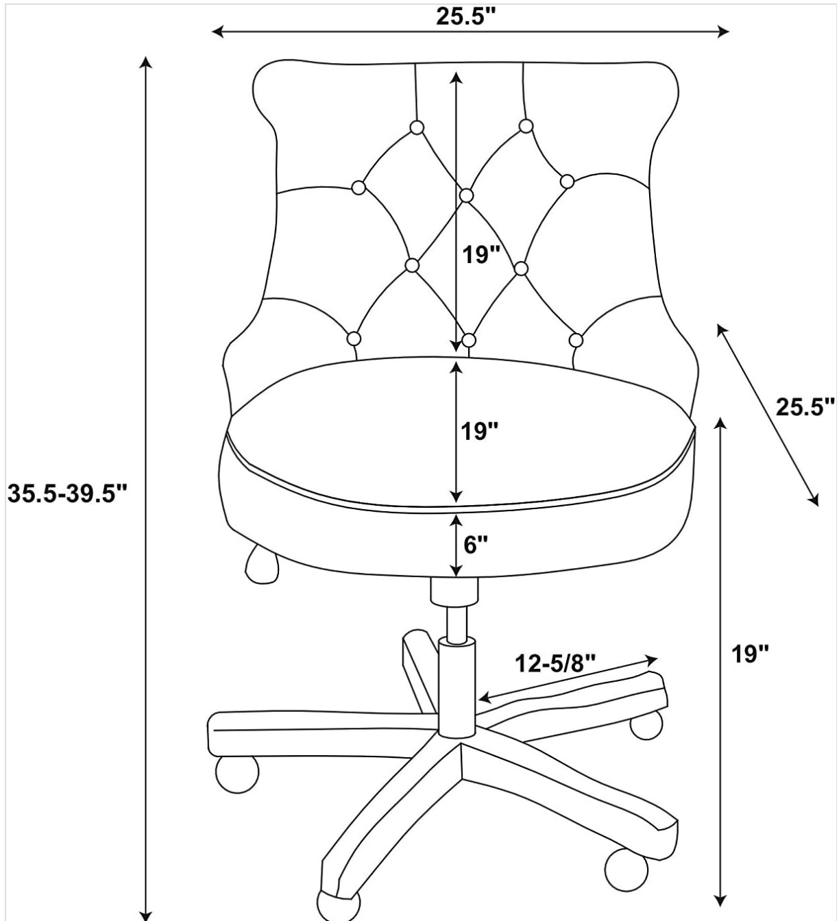
Image: Diagram illustrating the chair's dimensions and main components for assembly.
