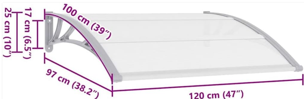
Image 4.1: Awning dimensions (120 cm width, 100 cm projection, 25 cm bracket height).
