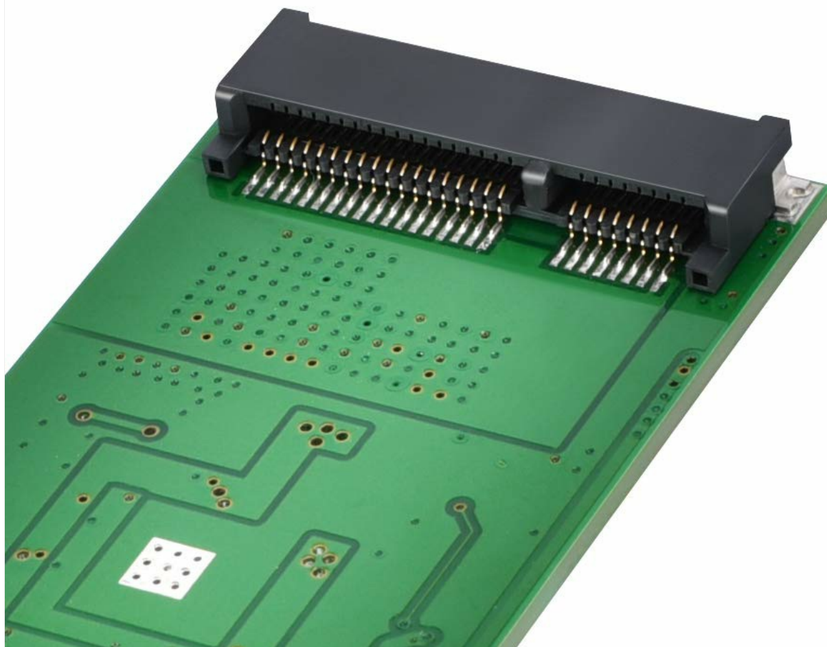
Image 2.1: Adapter showing mSATA SSD slot
