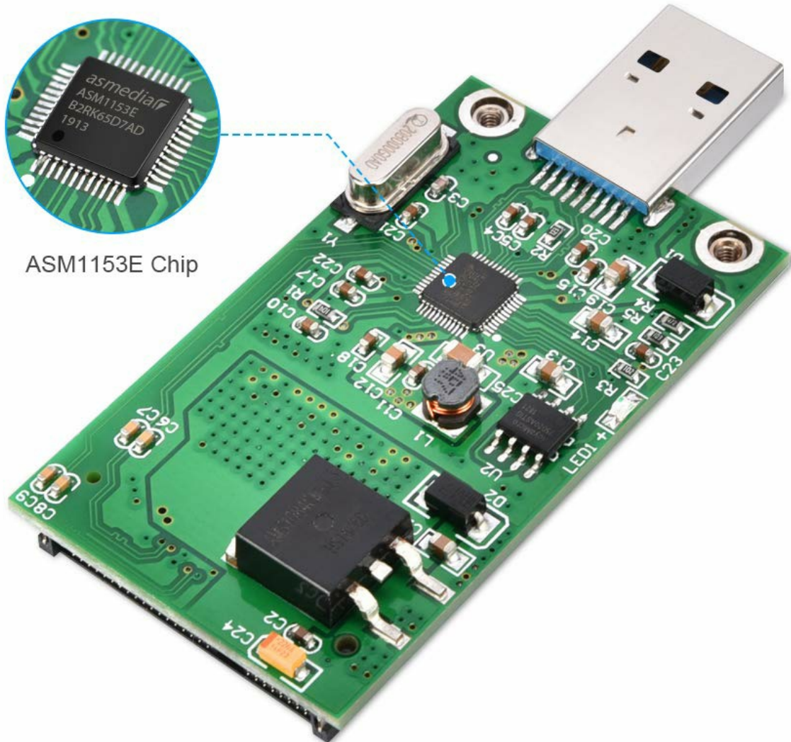
Image 8.1: ASM1153E Chip on the adapter board
