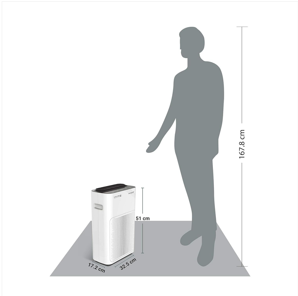
Image: Diagram showing the dimensions of the Aeroguard AP 500 (51 cm height, 17.2 cm depth, 32.5 cm width) relative to a human figure.
