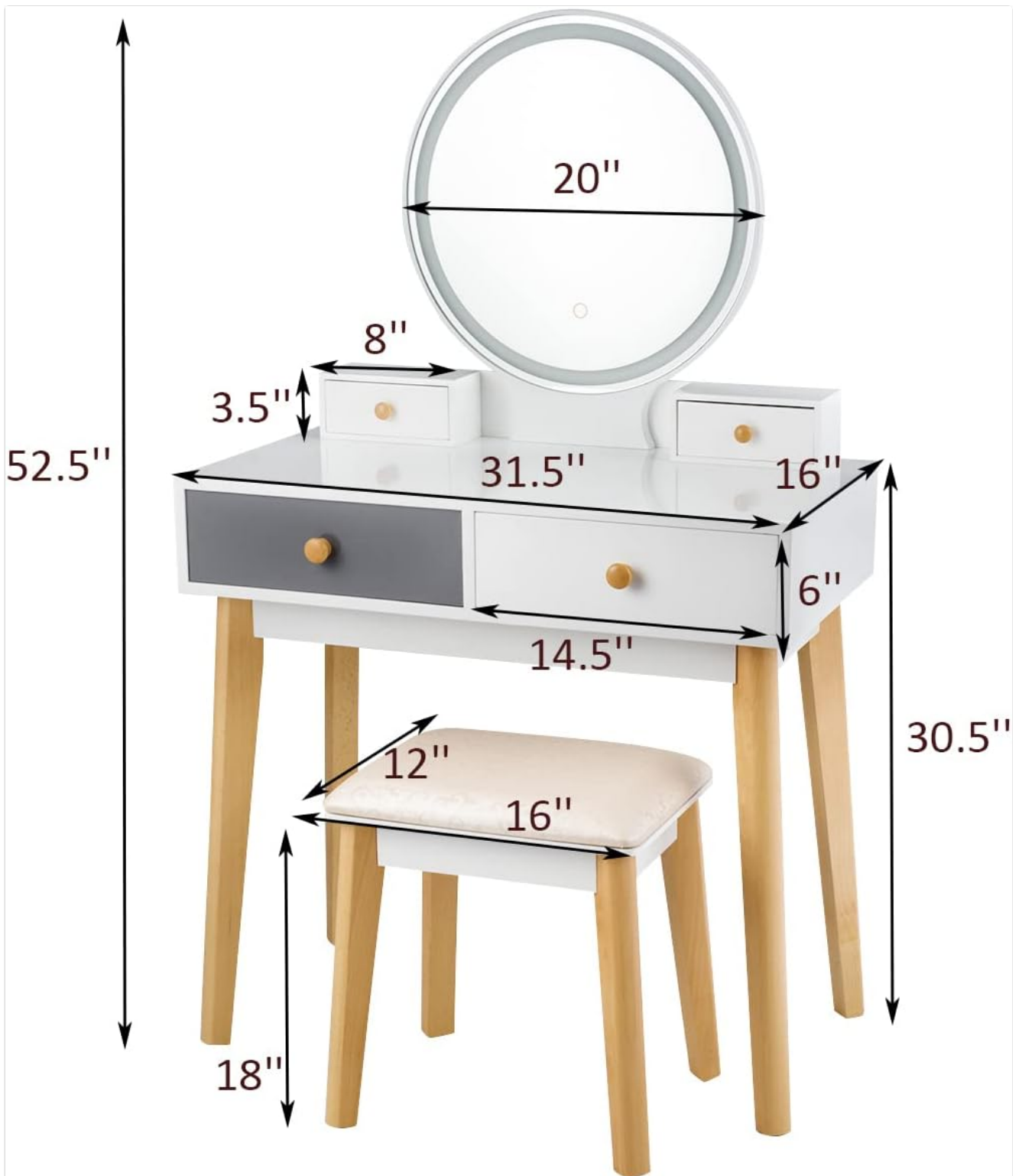
Image 2: Detailed dimensions of the vanity table and stool for proper placement and space planning.
