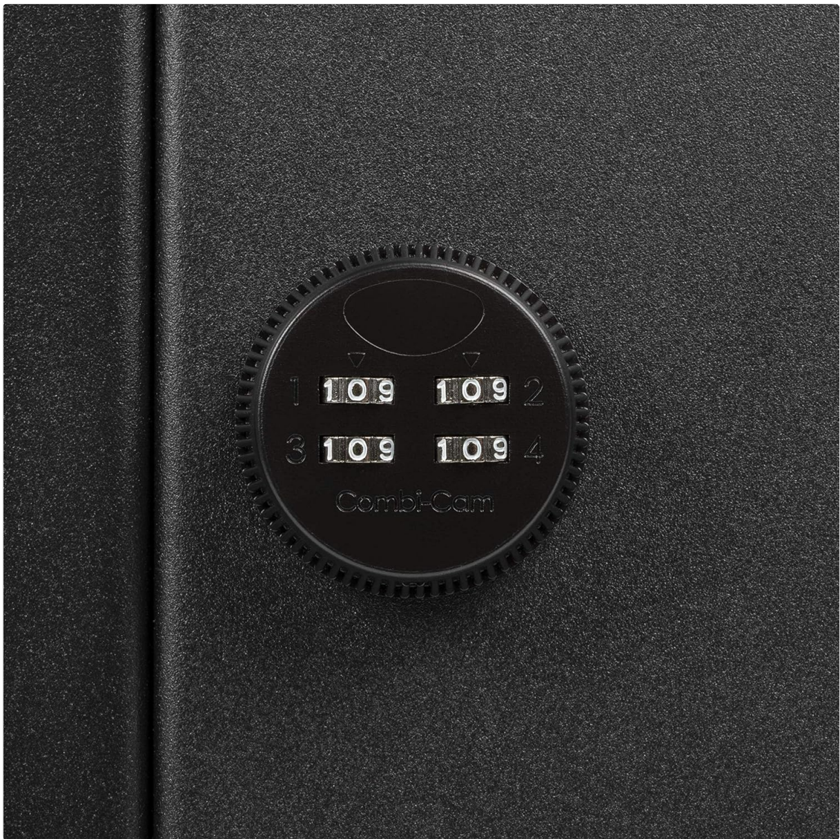
Image 5.1: A detailed view of the Combi-Cam combination lock, showing the four numerical dials for setting and entering the code.
