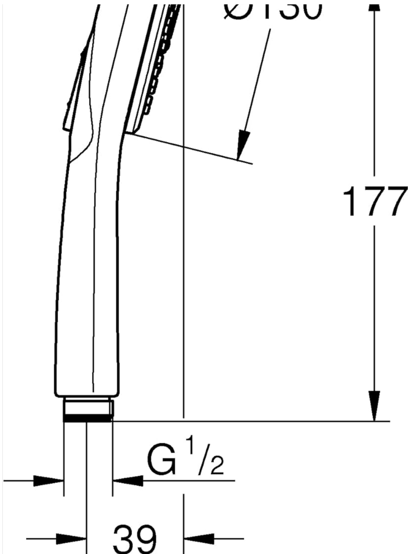
Figure 2: Technical drawing showing the dimensions and G 1/2 connection of the hand shower for proper installation.
