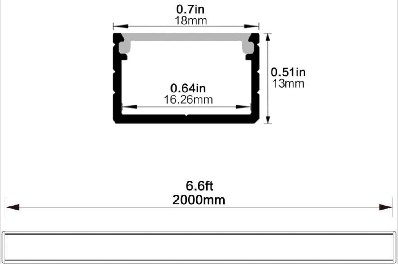
Image: A diagram illustrating the dimensions of the U-shape aluminum channel, including width, height, and inner space measurements.
