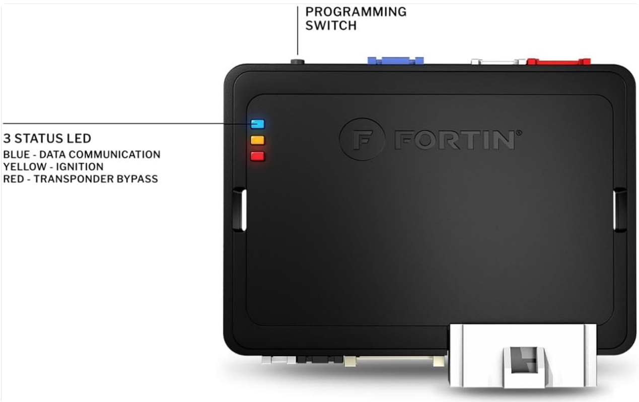
Image 6.1: A top-down view of the Fortin EVO-ONE module, clearly labeling the three status LEDs and their corresponding functions.
