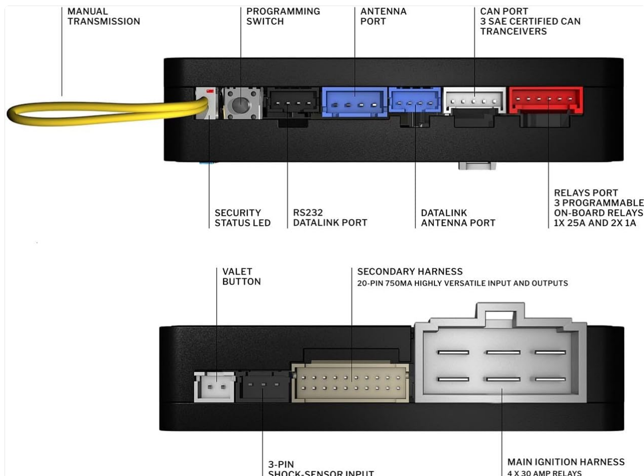
Image 4.1: A detailed diagram illustrating the various ports and connection points on the Fortin EVO-ONE module, including the programming switch, antenna port, datalink ports, and main ignition harness.
