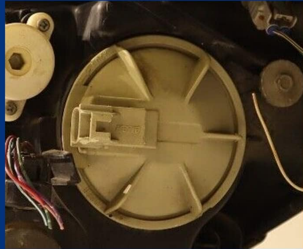
Image 5.1: Low Beam Bulb Connector Compatibility (Halogen vs. HID).
