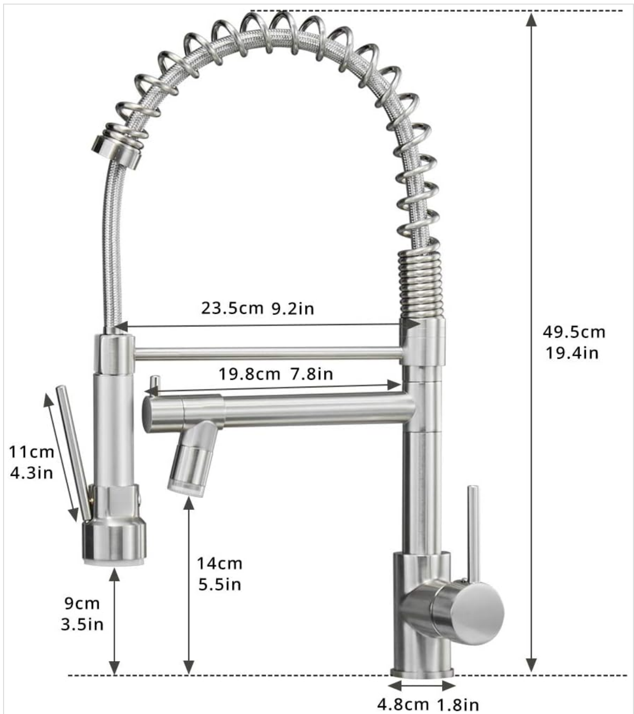
Image: Diagram showing faucet dimensions and pipe connection details.
