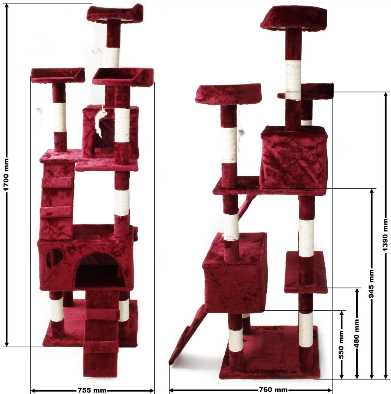
Figure 3: Front and side view assembly diagram illustrating the overall height (1700 mm) and width (755 mm, 760 mm) of the assembled cat tree.
