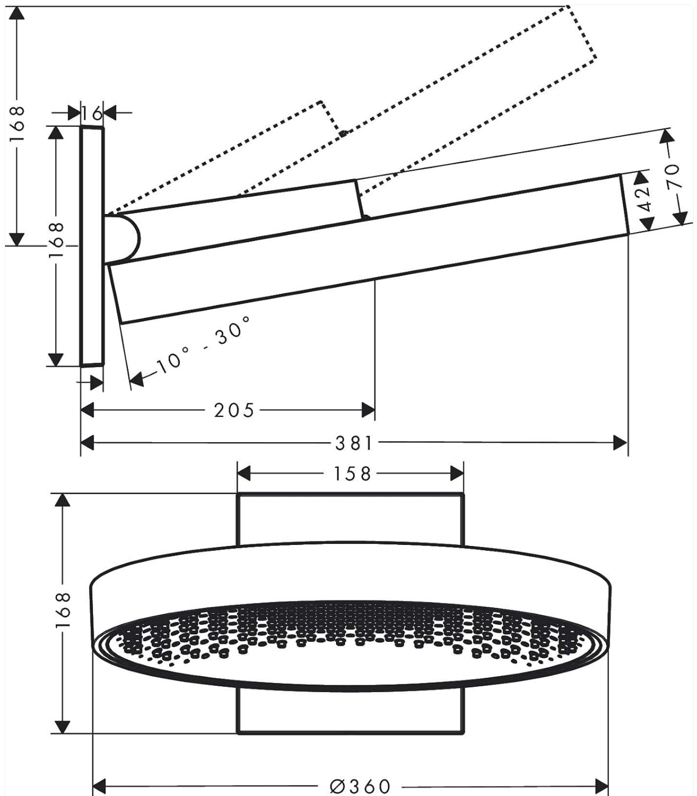
Image 2.1: Technical diagram illustrating the dimensions and adjustable angle range (10-30°) of the shower head and wall connector.
