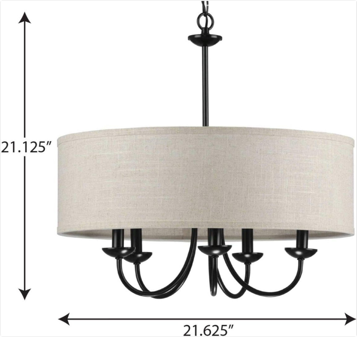
Image 4.1: Detailed dimensions of the chandelier fixture.
