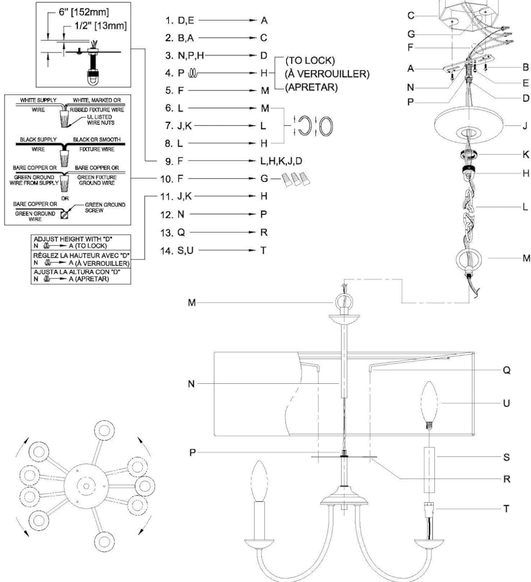
Image 5.1: Detailed assembly and wiring diagram for the chandelier.
