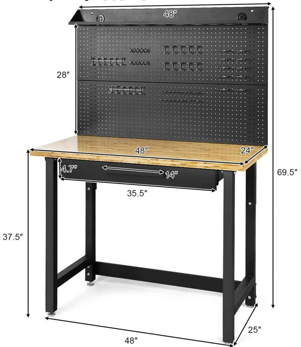
Image: A detailed diagram illustrating the dimensions of the Goplus workbench, including the overall height, desk height, tabletop length and width, and pegboard height.
