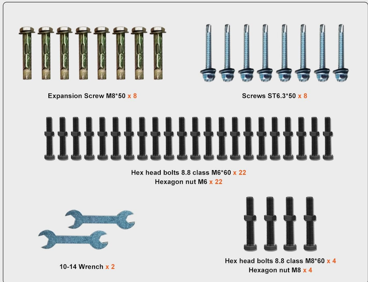
Figure 3.1: Complete Accessories for Installation
