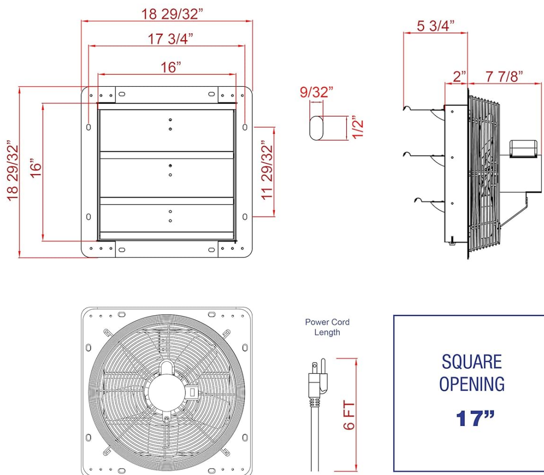
Figure 2: Detailed dimensions and specifications for the iLiving 16-inch Wall-Mount Shutter Exhaust Fan, including the recommended 17-inch square opening for installation.
