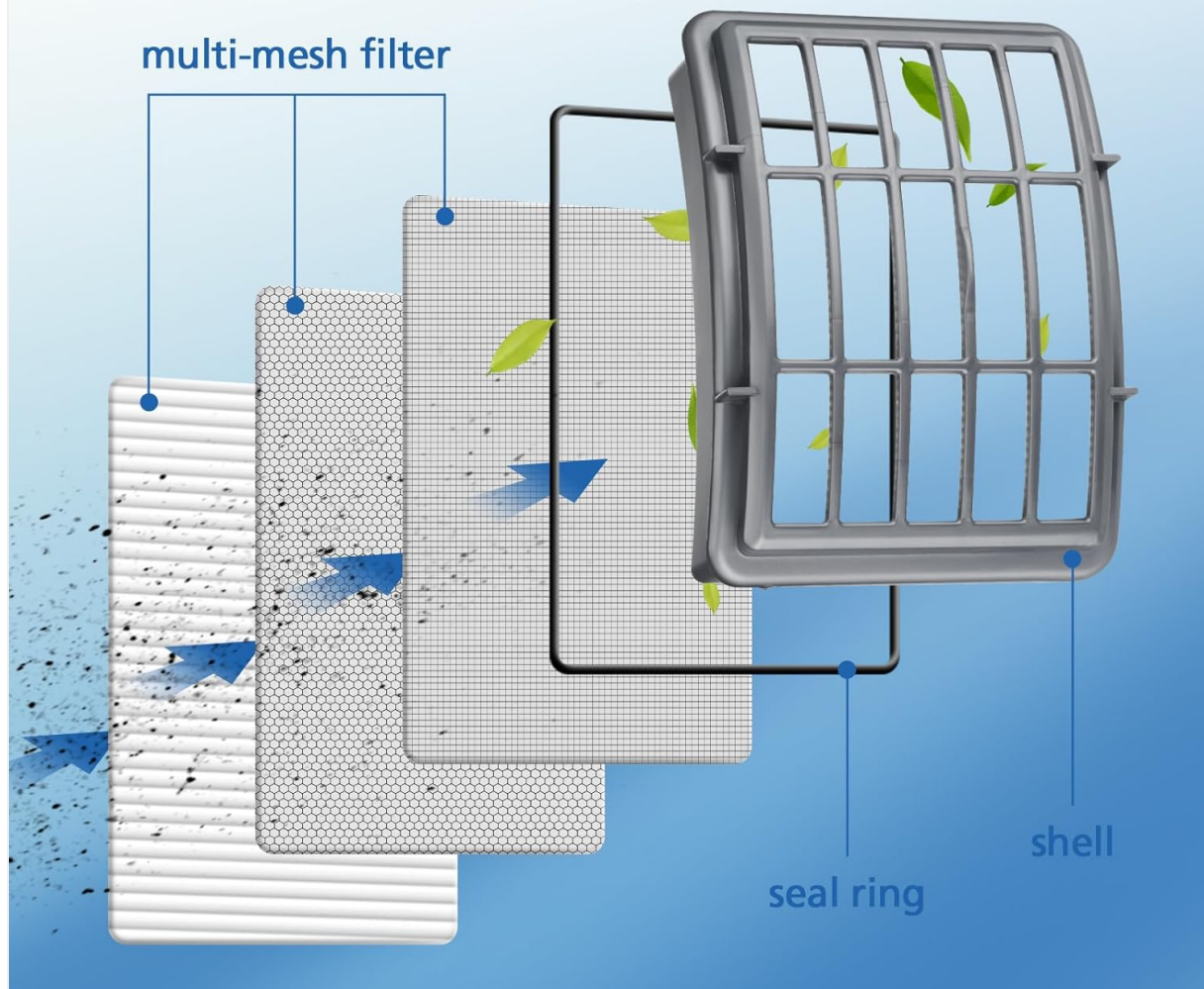
Image 5: Exploded view of the filter's multi-layer construction.
