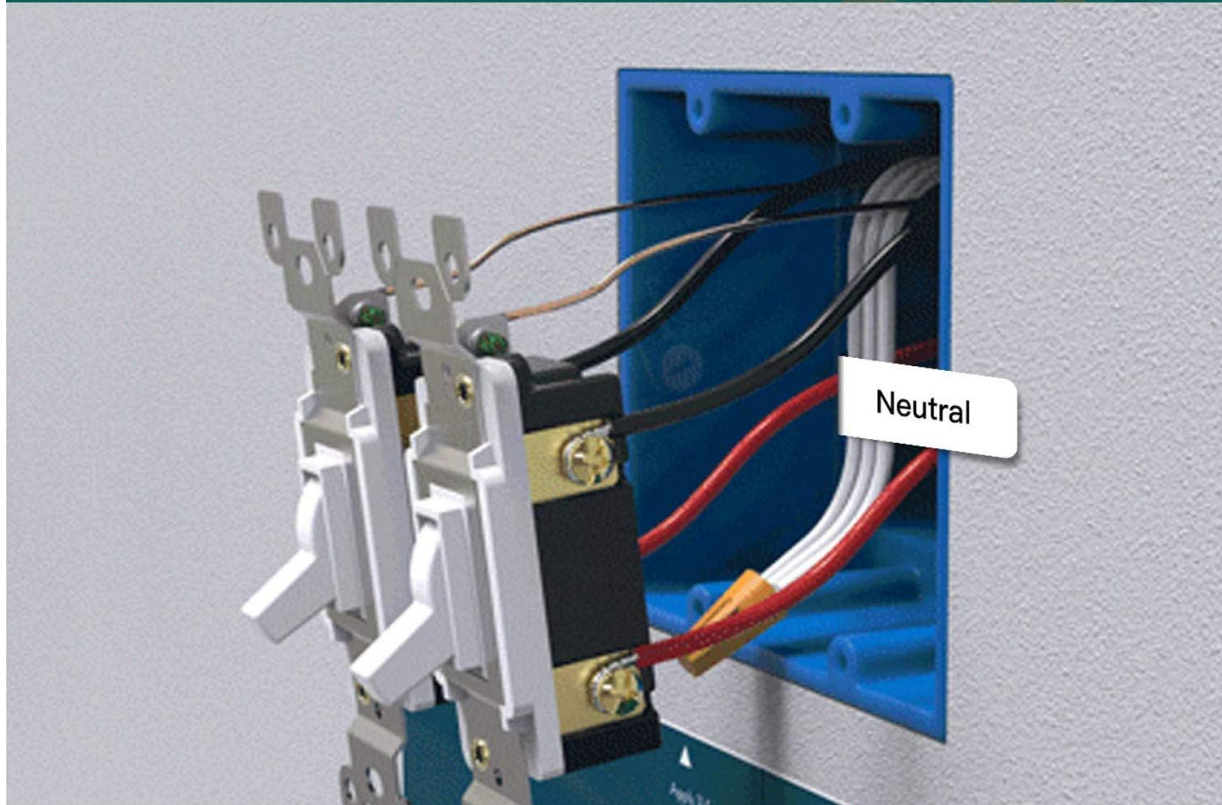
Figure 5.1: Identifying the Neutral Wire. This diagram shows a typical electrical box with a neutral wire (white) bundled, which is required for the smart switch installation.
