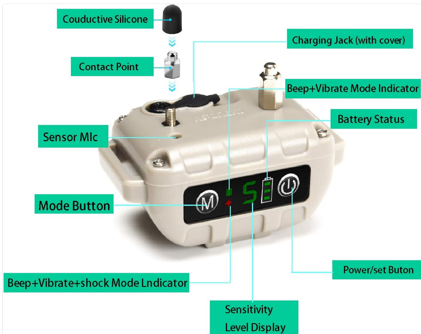
Image 2: Diagram illustrating the various components of the Trulrox Bark Collar receiver, including the charging jack, contact points, sensor microphone, mode button, power/set button, sensitivity level display, battery status, and mode indicators.
