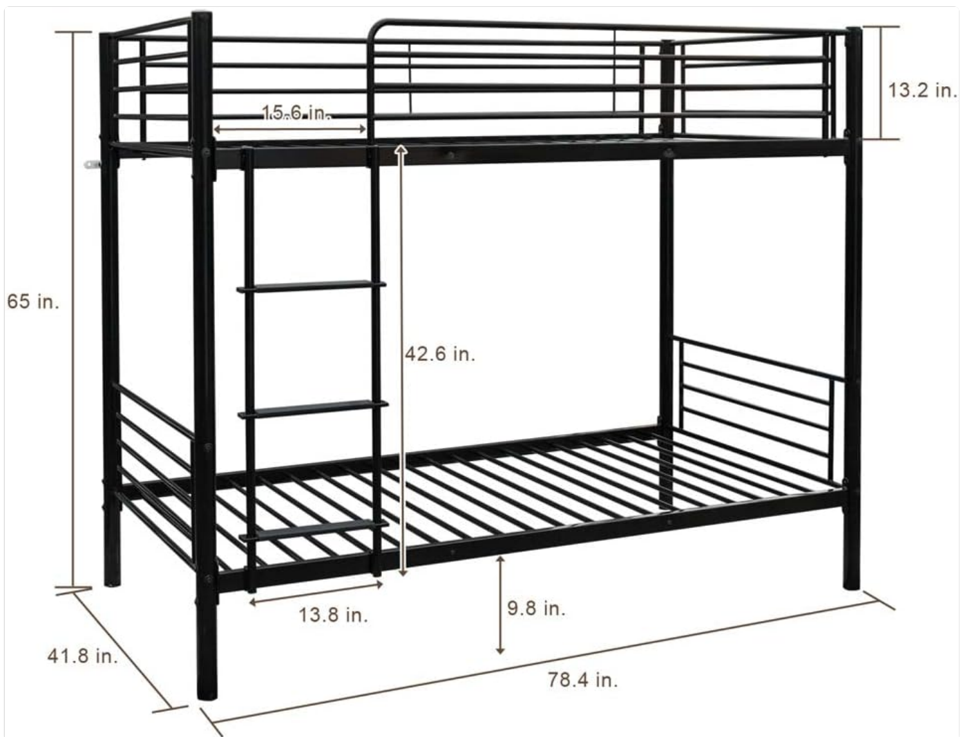
Image: Detailed diagram showing the dimensions of the FCH Twin Over Twin Metal Bunk Bed, including overall height, width, length, and distances between bunks and guardrail height.
