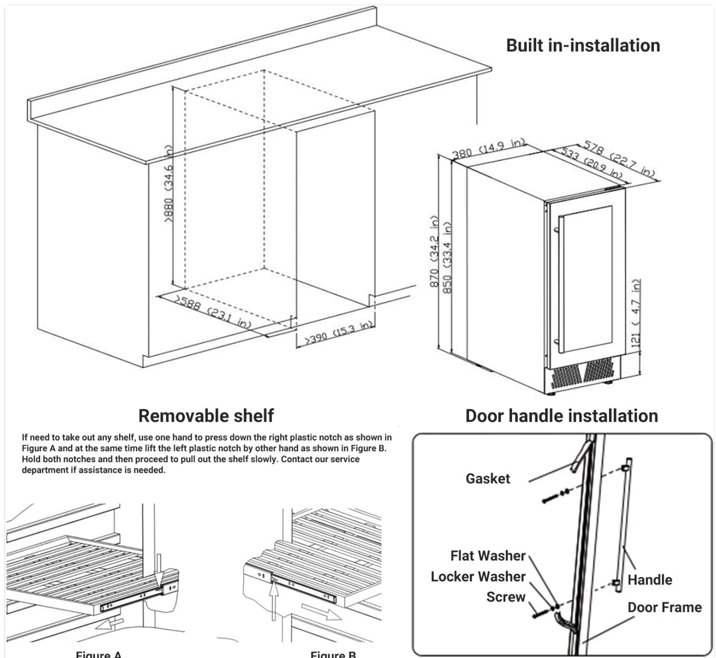
Figure 2: Installation guidelines for the wine fridge, including dimensions for built-in placement and instructions for removing shelves. The unit features front
