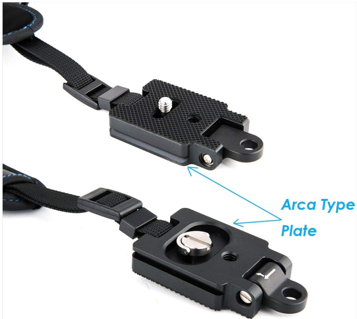
Figure 2.2: Detailed view of the Arca-Type base plate.
