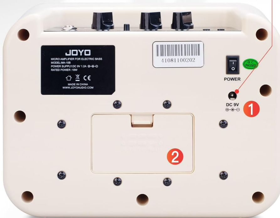
Image 3.1: Rear panel of the MA-10B, illustrating the power adapter input and battery compartment.
