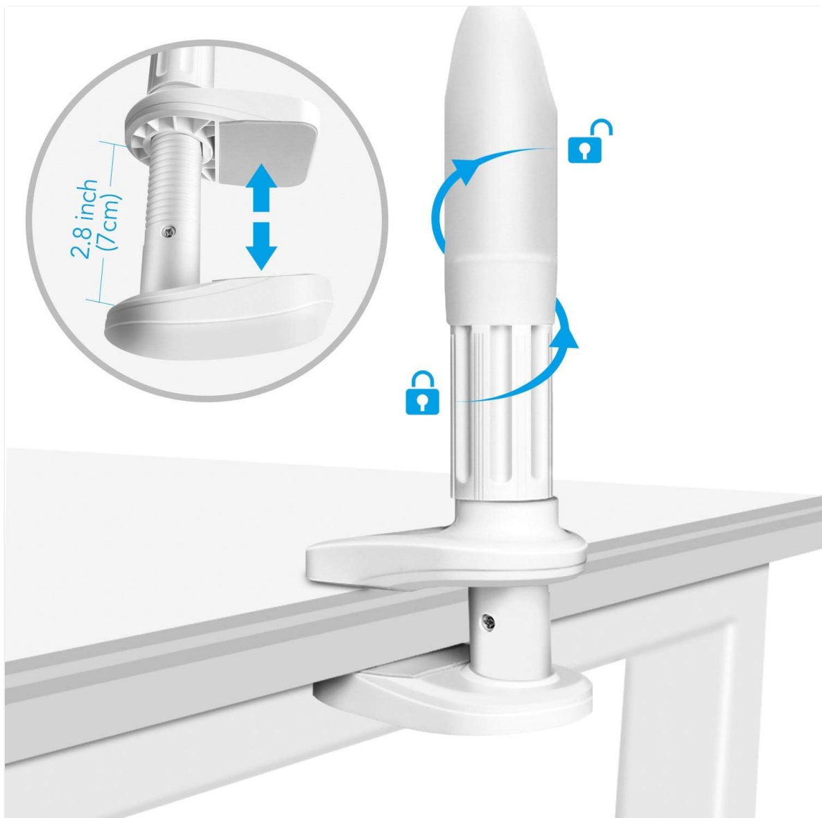
Image: The clamp mechanism of the mount, showing how it attaches to a surface up to 2.8 inches thick.
