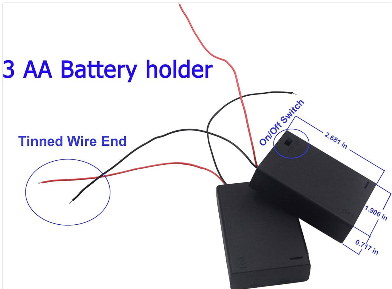
Image: A 3-cell AA battery holder with its ON/OFF switch clearly visible on the side, along with the red and black tinned wire leads extending from it. Dimensions are also indicated.
