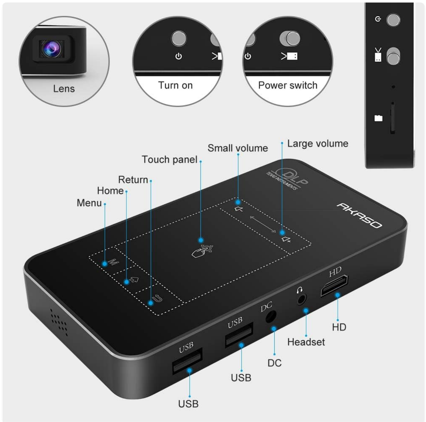
Image: Detailed view of the AKASO WT50 Mini Projector, highlighting its various ports (USB, HDMI, DC, Headset) and control buttons (Touch panel, Home, Menu, Volume, Power switch, Lens focus dial).
